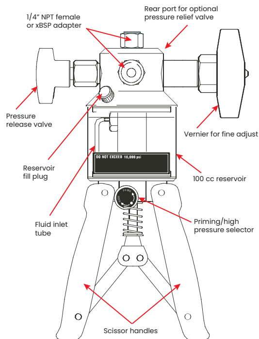
PV212-X components
